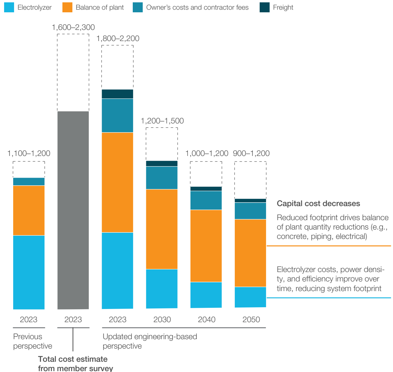
Renewable H 2 capex (US Gulf Coast 1 GW alkaline facility example), USD/kW, for fully installed system
